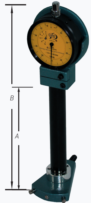
Vertical, Style 3 For vertical axis bores at eye level; best choice for bench inspection applications.
